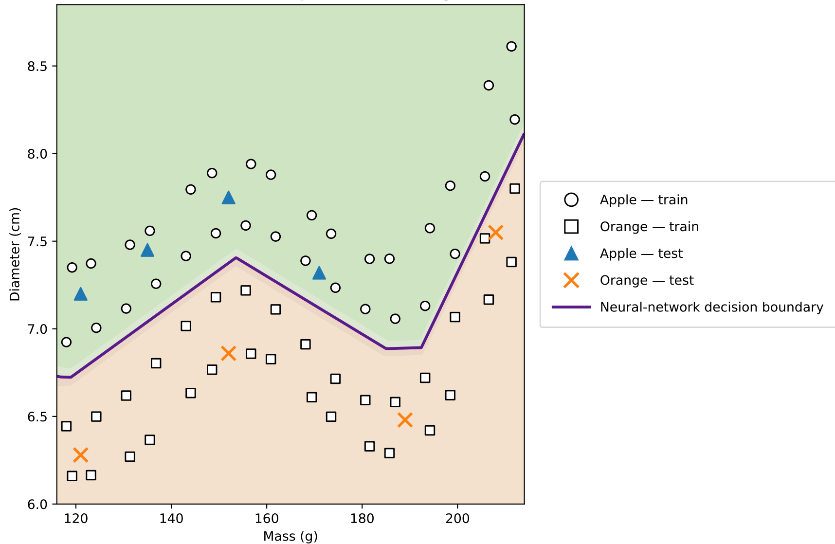
Neural network output after training
